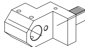
Toolholder for boring bar
