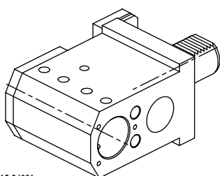
Combi toolholder for boring bar and insertdrill ø40 mm
