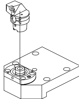
Face and O.D. cutting holder HSK 40 A+C
