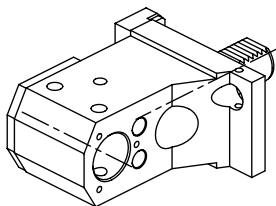
Combi toolholder for boring bar and insertdrill
