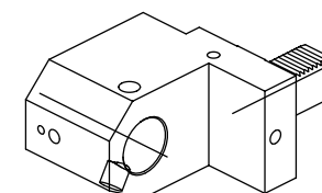
Toolholder for insertdrill
