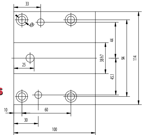
Drill socket 114-34015 <MT1> 114-34016 <MT2> 114-34017 <MT3>
