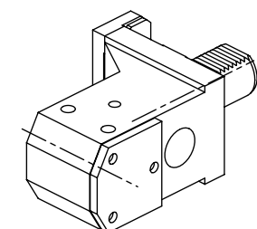
Combi toolholder for boring bar and insertdrill ø40 mm
