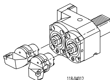
Face and O.D. cutting holder HSK 40 A+C
