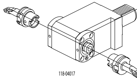
Boring bar holder
