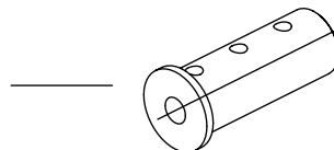
Boring bar sleeve and throw-away drill socket K114354 (Ø10 mm) K114355 (Ø12 mm) K114356 (Ø16 mm) K114357 (Ø20 mm) K114358 (Ø25 mm)
