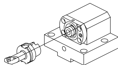
Boring bar holder HSK 40 A+C
